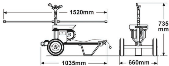
RI 10 ...Mass: 80 kg (including hose)
